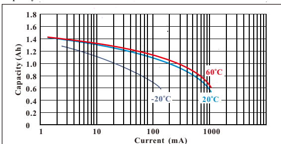
Capacity vs Current Characteristics
